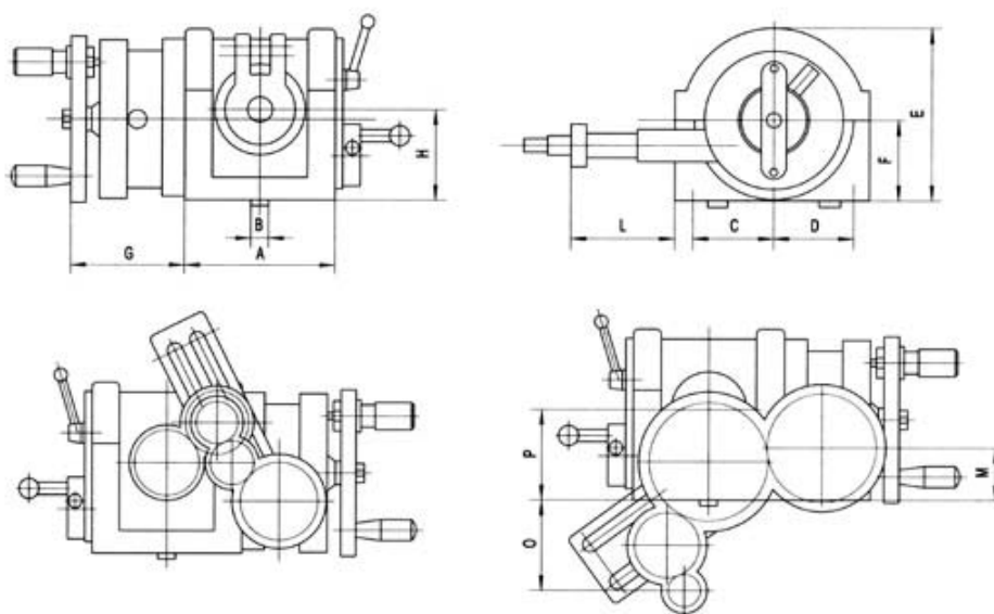
FW80 Installationsketch and dimensions
