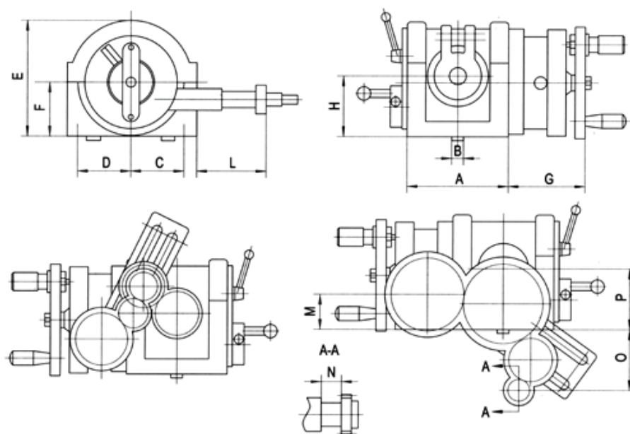
Dimensional Sketch
