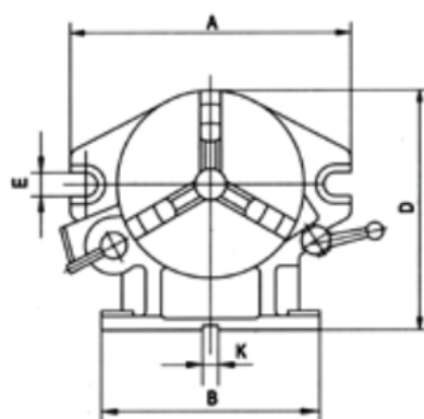
Installation sketch and dimensions
